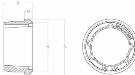
W Style TB Bushing Weld-On Hubs
